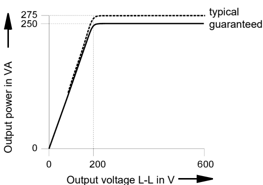
Single-phase operation L-L
