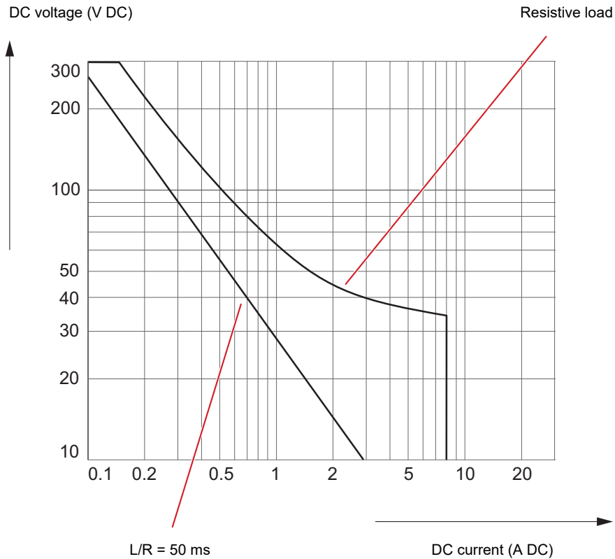
Load limit breaking capacity curve for binary output relays with DC voltages
