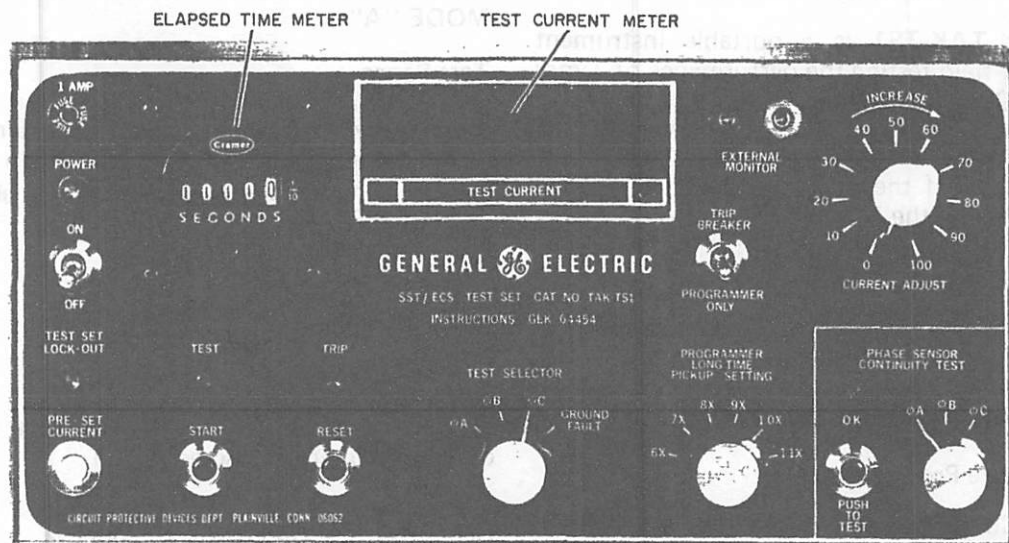
Fig. 1. Front panel of Test Set TAK-TS1
