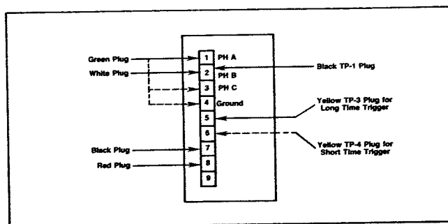
Figure 11. Test Connections—Models 4WAG and 4WDG
