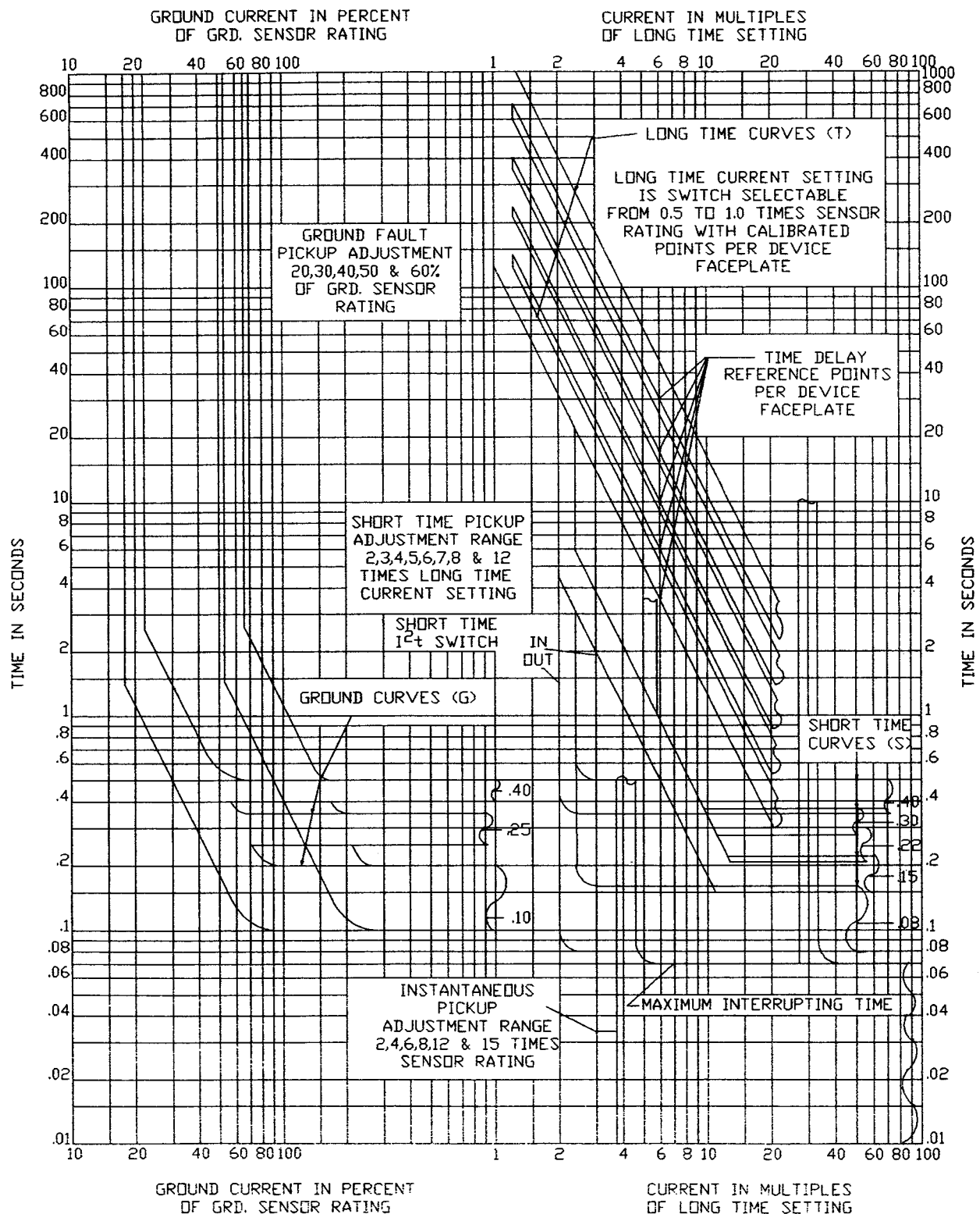
Figure 5. Time Current Curves—Static Trip III
