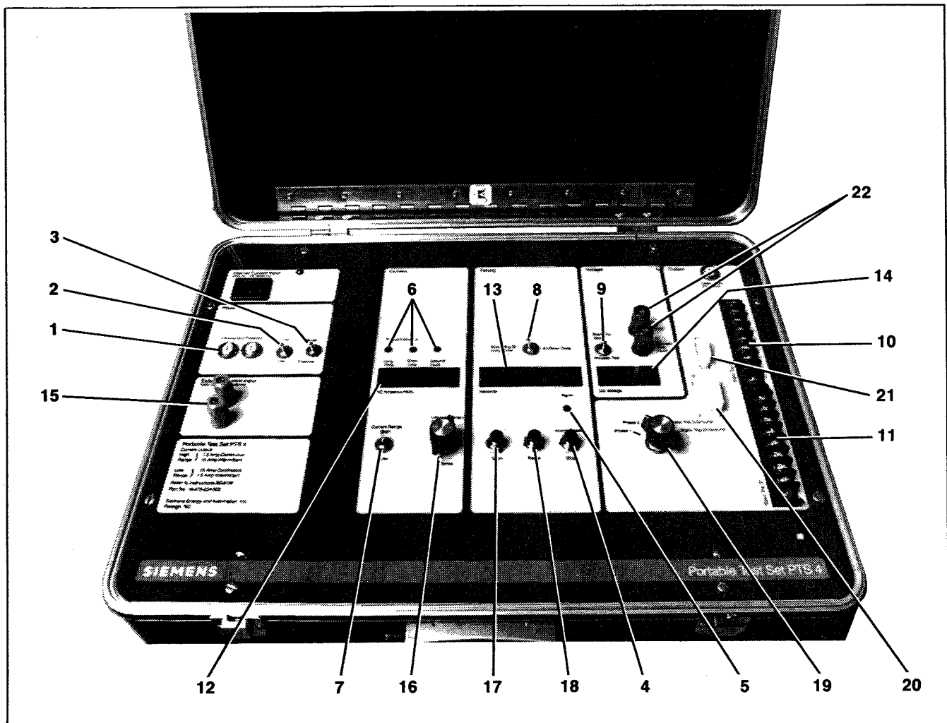
Figure 3. Control Panel
