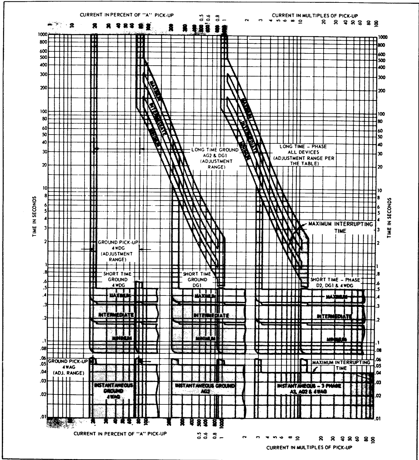
Figure 15. Time Current Curves—Models A2, A3, D2, DG1, 4WAG and 4WDG
