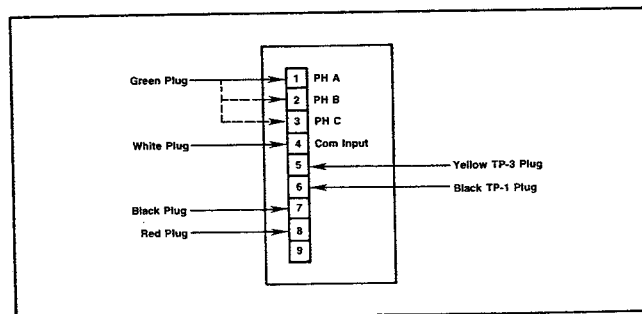
Figure 10. Test Connections—Models AG, AG1, AG2, DG and DG1
