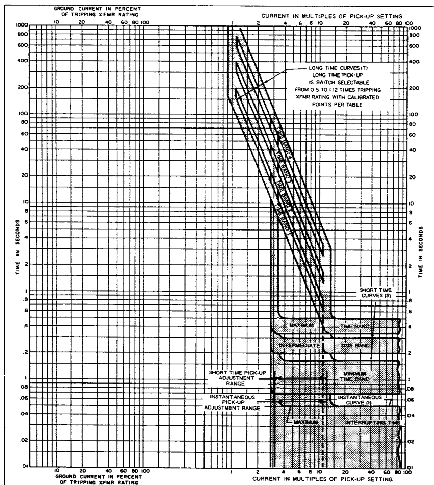
Figure 20. Limitrip Time Current Curves
