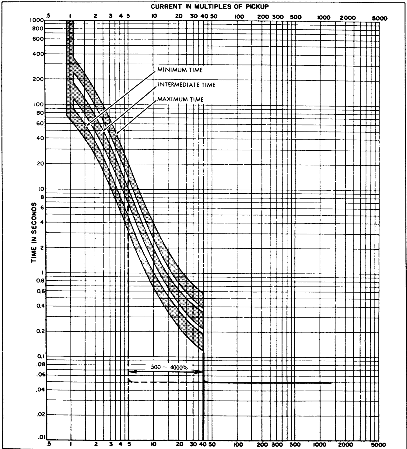
Figure 17. Time Current Curves—Model C3
