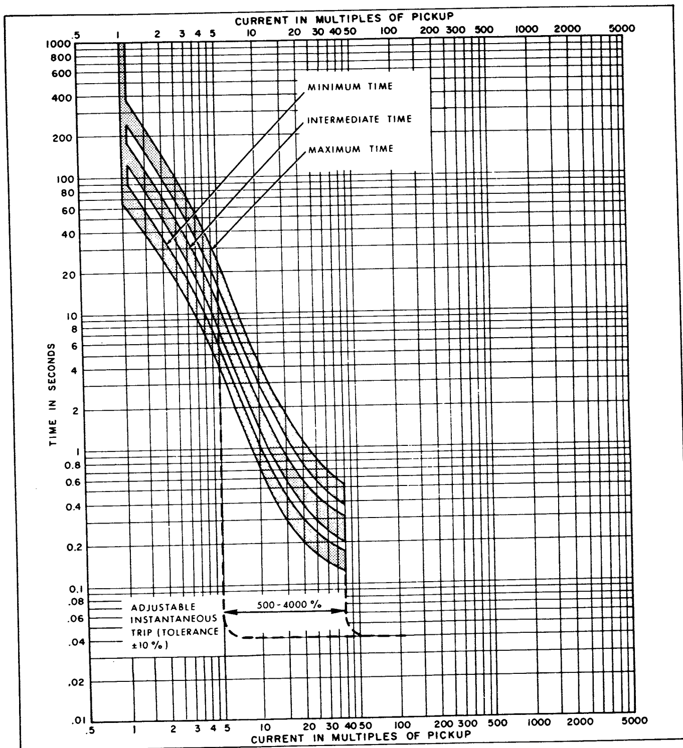
Figure 16. Time Current Curves—Models C, C1 and C2
