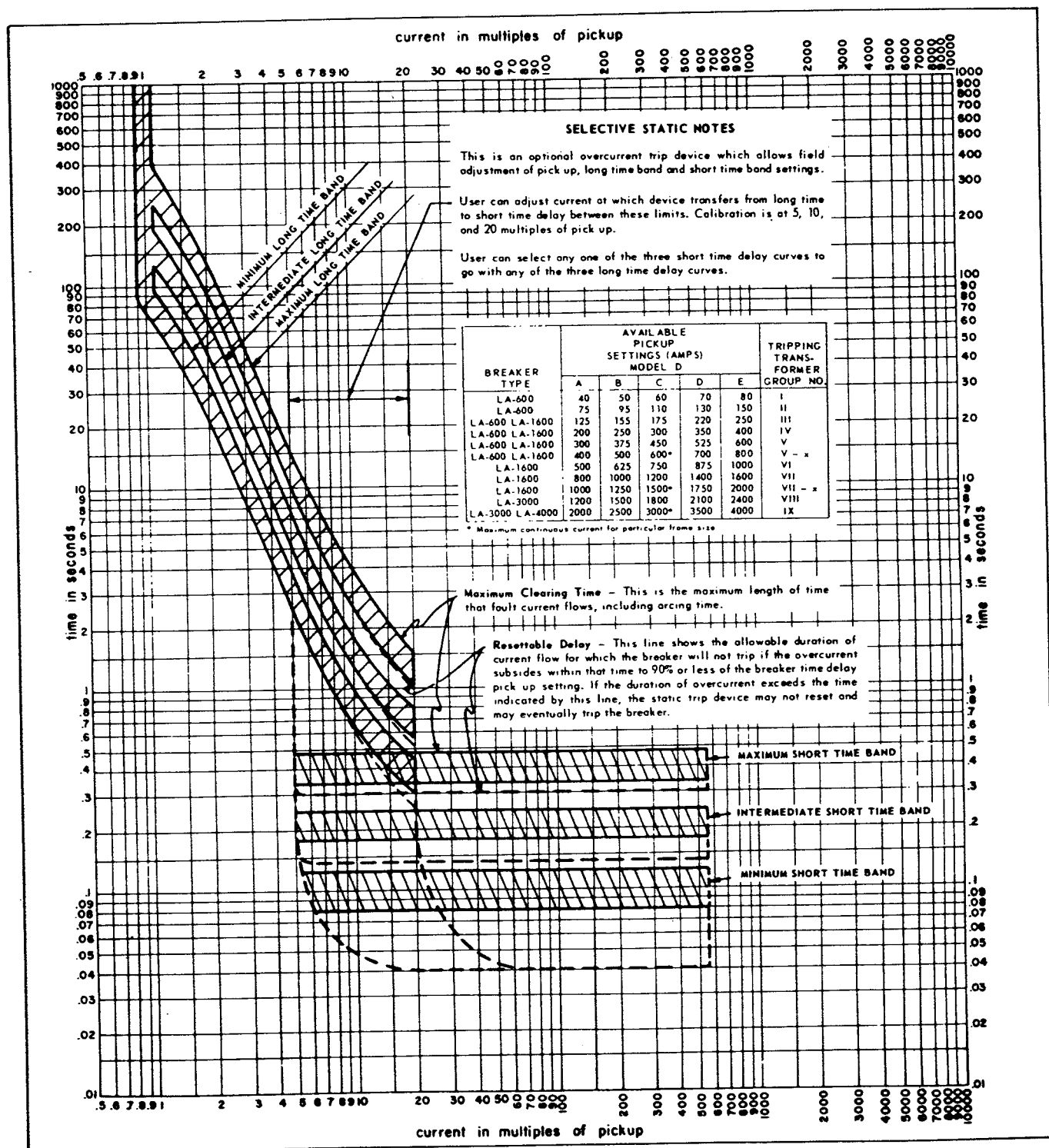
Figure 14. Time Current Curves—Models D and D1
