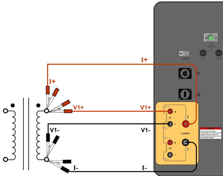
Figure 4. Typical Single Phase TRM Connections
