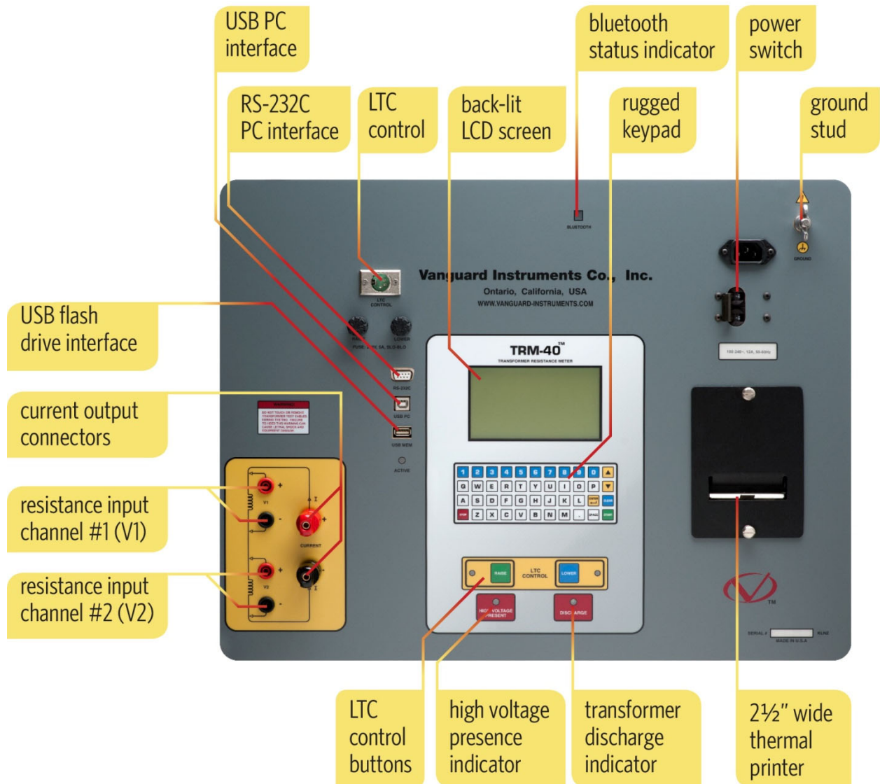
Figure 1. TRM-20/40 Controls and Indicators
