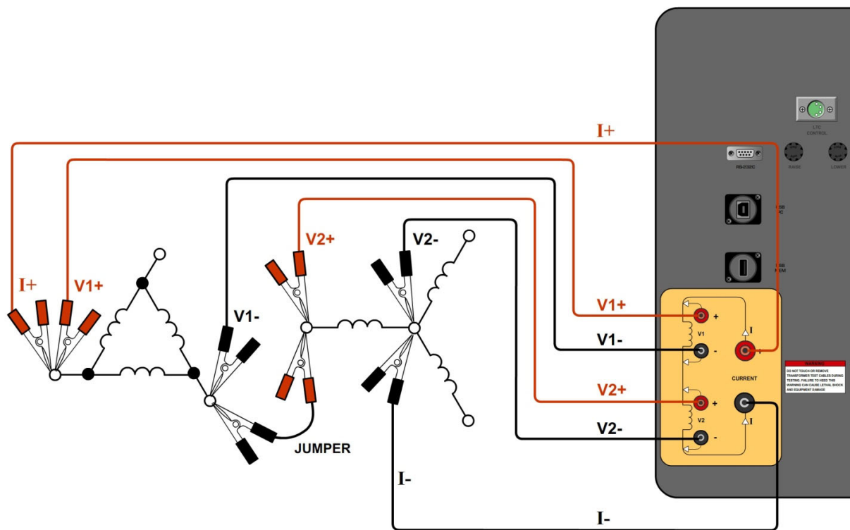
Figure 5. Typical TRM Connections Diagram for 2 Windings
