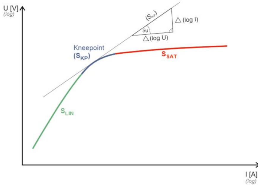
Figure 2.2: Excitation diagram
