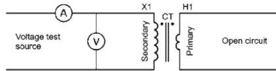
Figure 2.3: Excitation measurement setup
