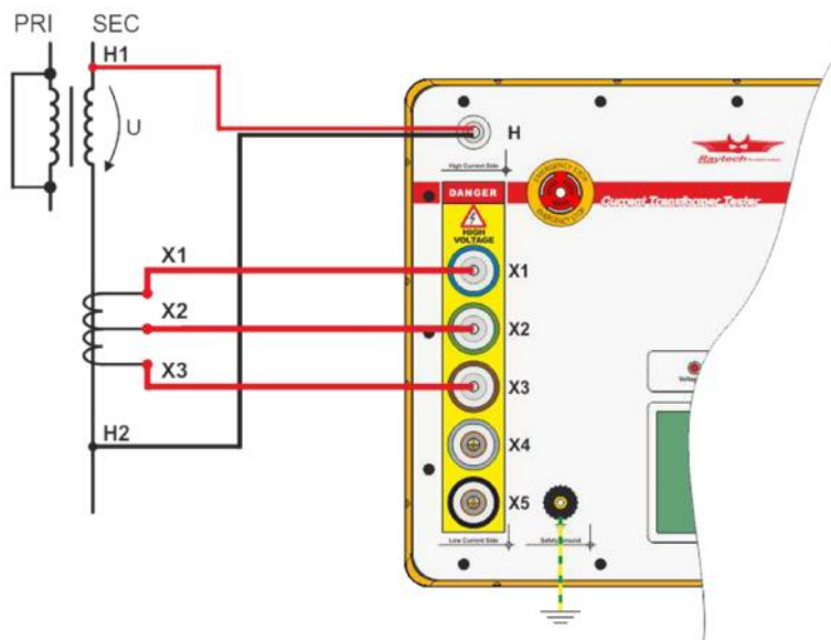
Figure 3.1: Example measurement with a built-in three taps CT under test connected to the power transformer on the secondary winding. The primary winding of the power transformer is short circuited to prevent any voltage U on the secondary winding of the power transformer.
