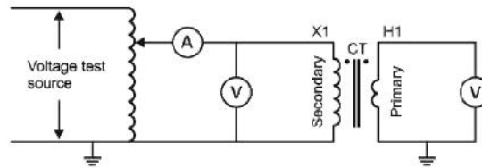
Figure 2.4: Turns ratio measurement setup
