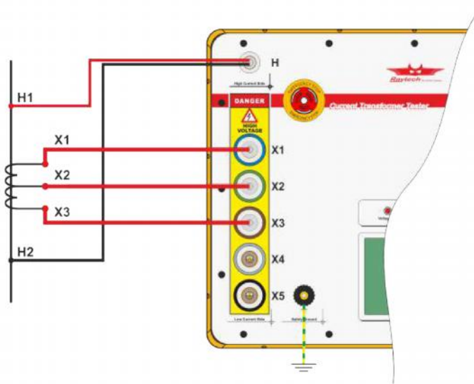
Figure 1.1: Example measurement with a three taps CT under test connected to the power transformer on the secondary winding. The primary winding of the power transformer is short circuited to prevent excess voltage.
