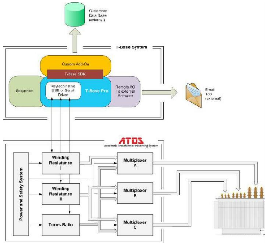
Figure A.2: T-Base Pro application example
