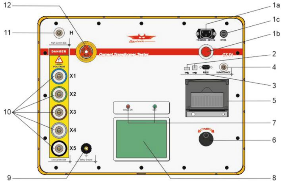
Figure 4.1: Overview of the CT-T1's operation elements
