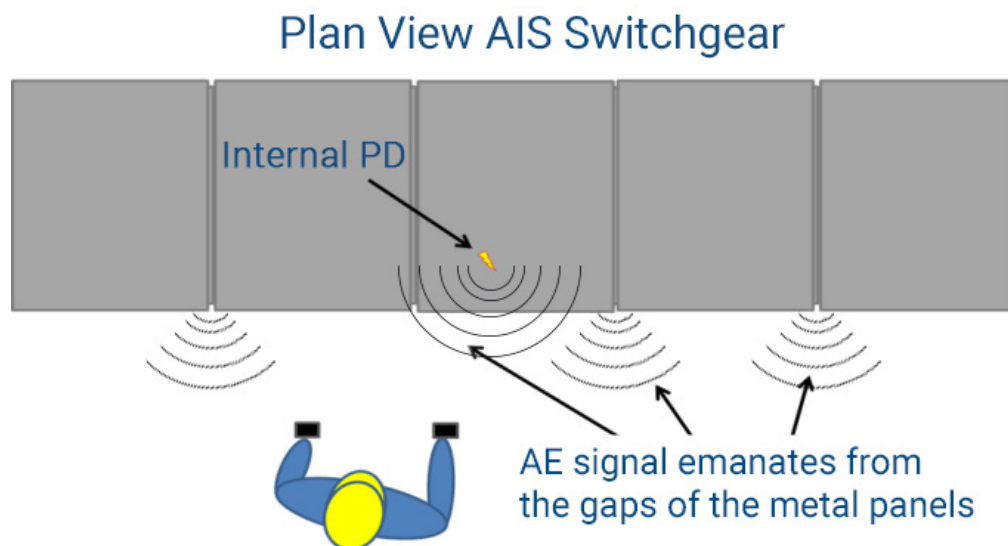
Figure 2: PD pulse propagation in AIS panels
