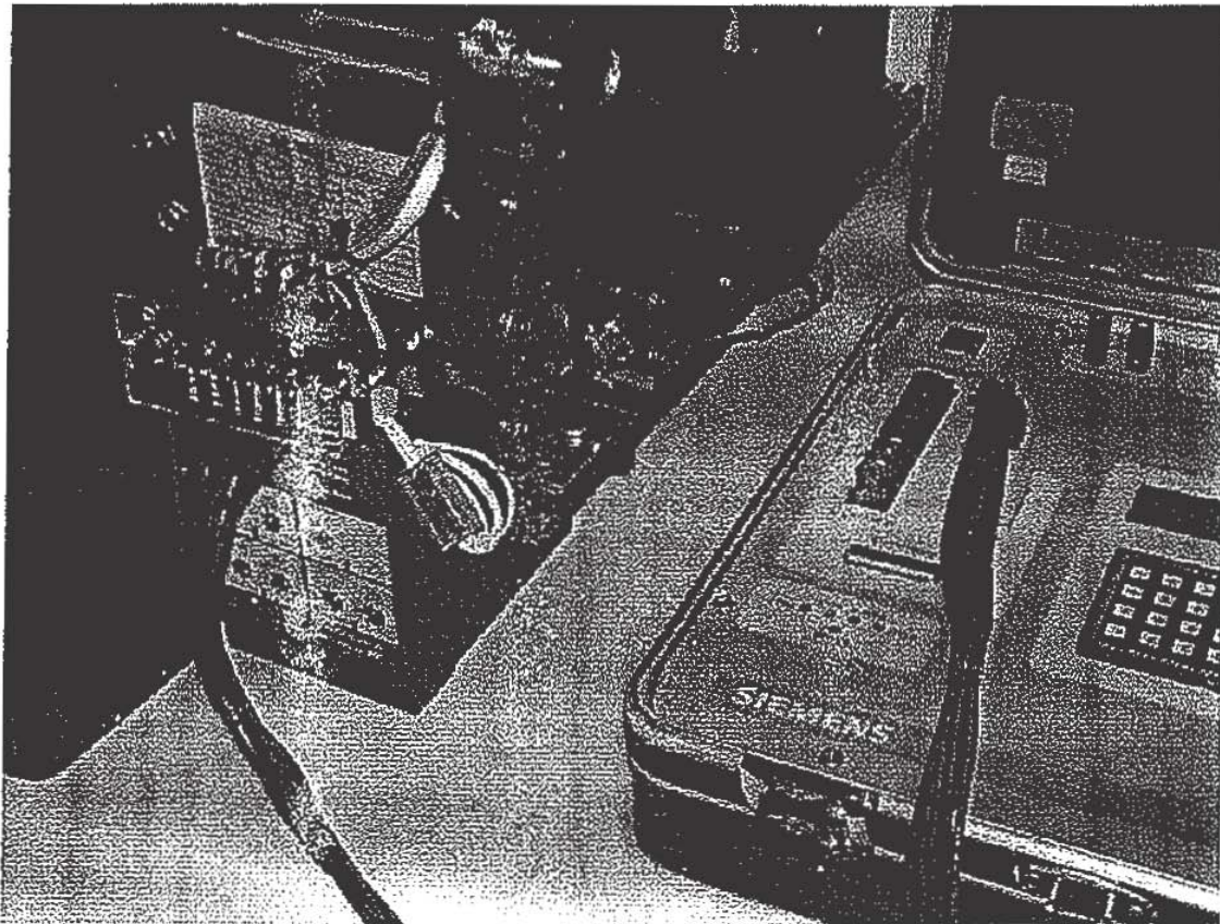
Figure 2 Attachment of the test cable to an STIII mounted on a breaker
