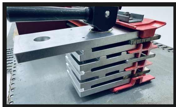
I-Line Cam Clamp in use
